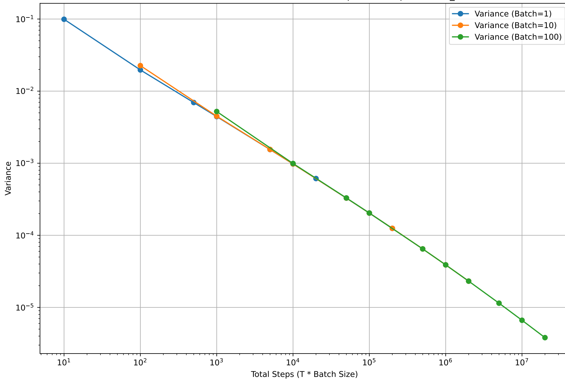
Slock Biases and Variances for Different Batch Sizes; \alpha=1.1 . optiized eta_star for each T
